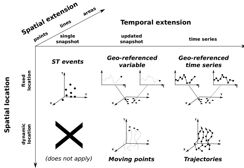
Fig. 1 Context for ST Clustering
